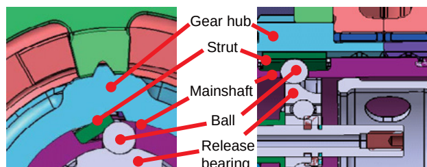
Fig. 5 Overrun state
