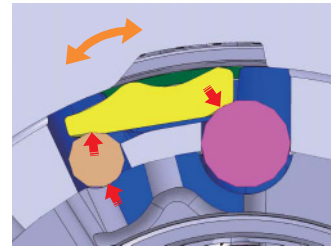
Fig. 14 Neutral state
