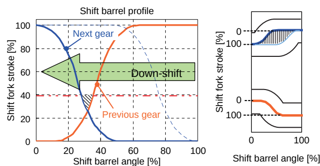
Fig. 7 Down-shift shift barrel profile
