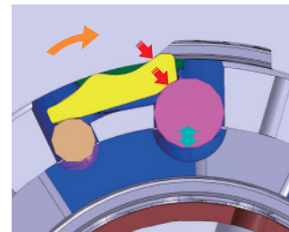
Fig. 15 One-way state
