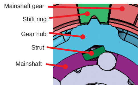
Fig. 3 Up-shift state
